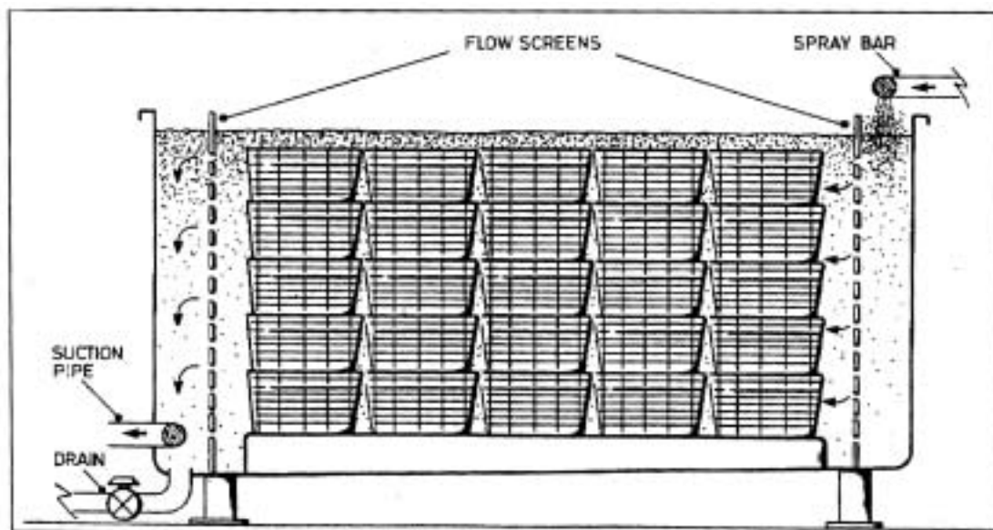
Side View of Multi-layer System
