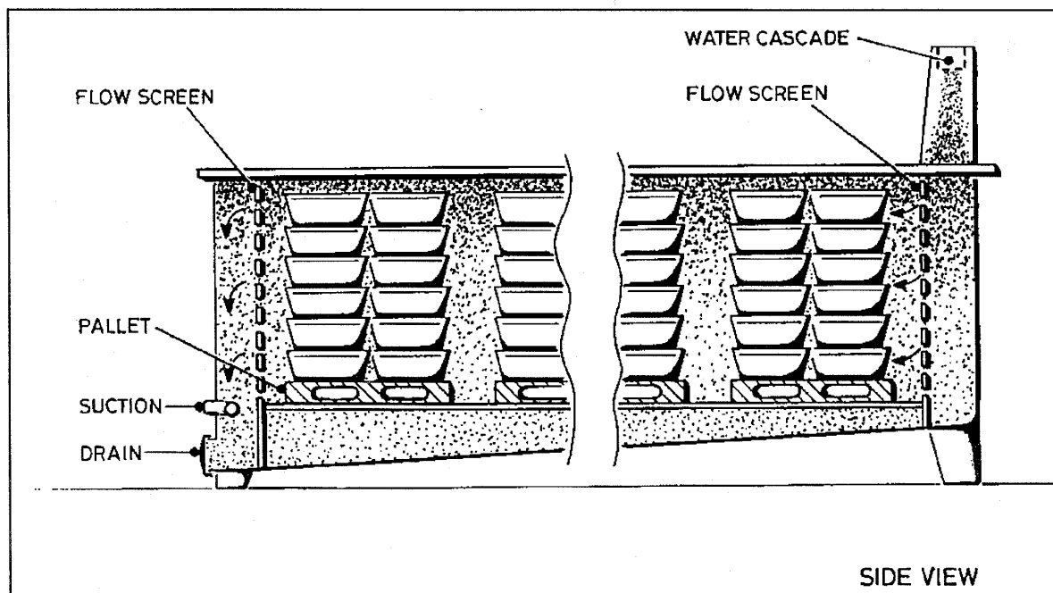
Side view of a multi-layer system
